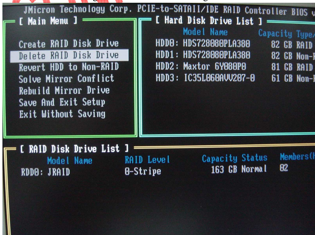
Figure 13. Delete RAID Dialog Box 1
